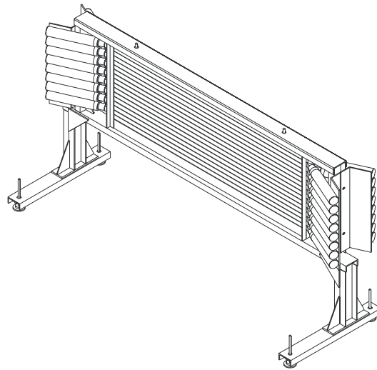
Figure 2.6: Sketch of the horizontal hodoscope.
