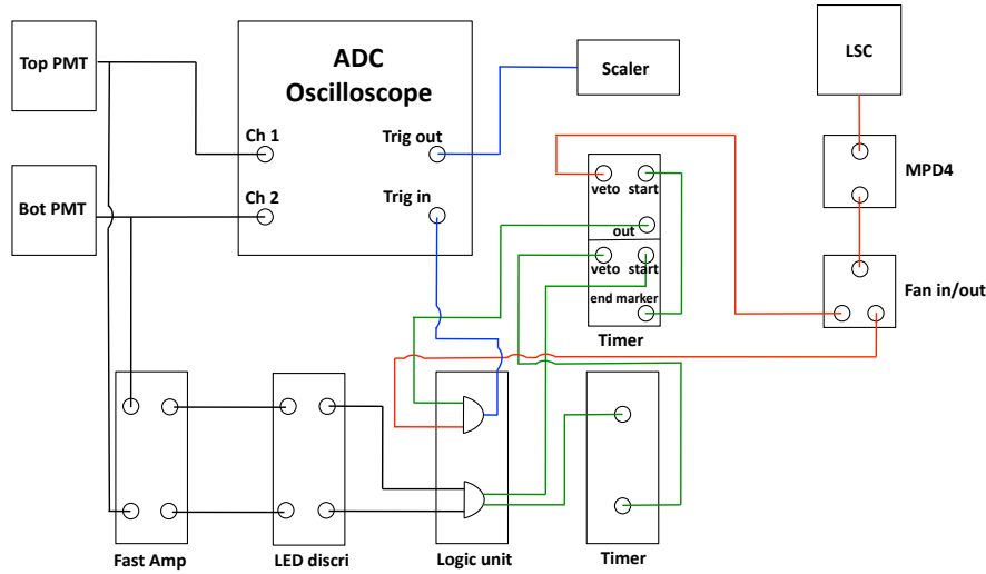
Figure 4.1: Schematic of the DAQ system.
