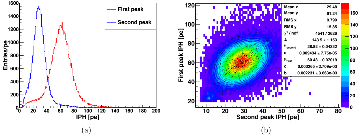
Figure 4.20: Left: the integrated pulse height of the first peak (red) and the second peak (blue) using the peak finding algorithm. Right: a 2D histogram of the integrated pulse height of the two peaks showing the correlation.
