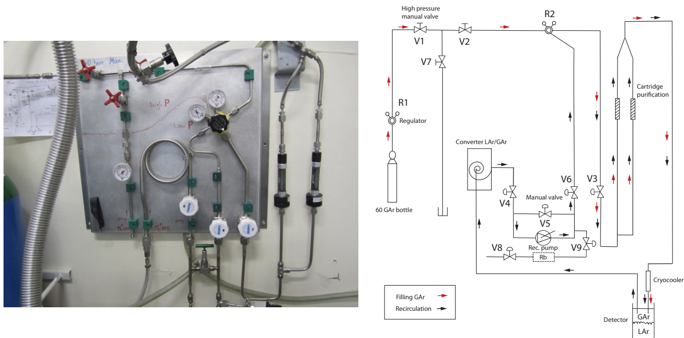
Figure 3.27: The gas system responsible for Ar filling, recirculation and purification. The arrows show the direction of Ar during filling in red, and during recirculation in black.
