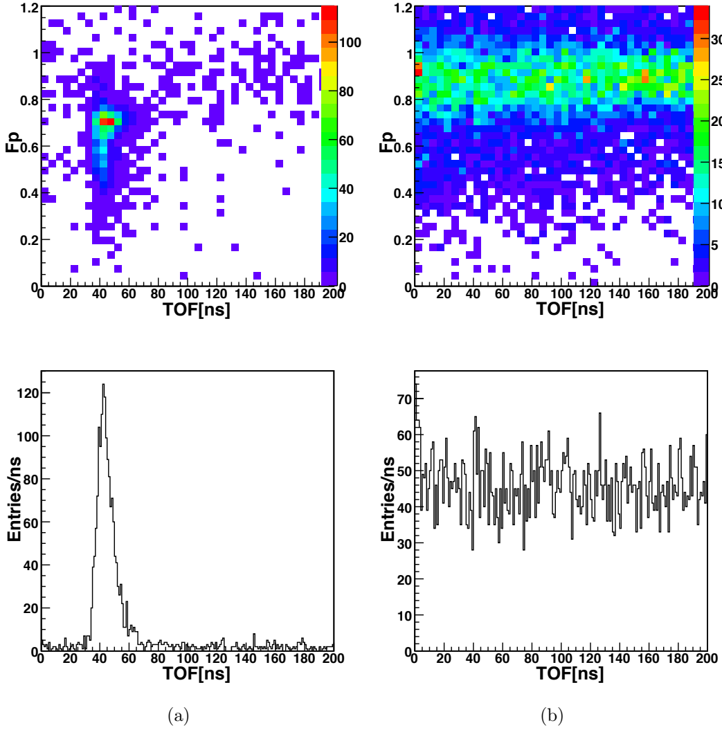
Figure 3.19: Ratio F_p vs. time of flight (TOF) in the 3'' LSC and its corresponding TOF projection after applying the F_p cut in the 5'' cell at 40^\circ . A typical neutron TOF is displayed in (a) for F_p < 0.75 , while (b) shows the TOF distribution after selecting the electronic recoils band in the 5'' cell.
