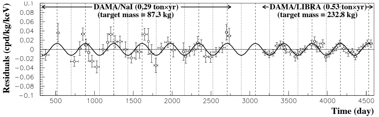
Figure 1.8: Annual modulation between 2 and 6 keV taken by DAMA collaboration [58].
