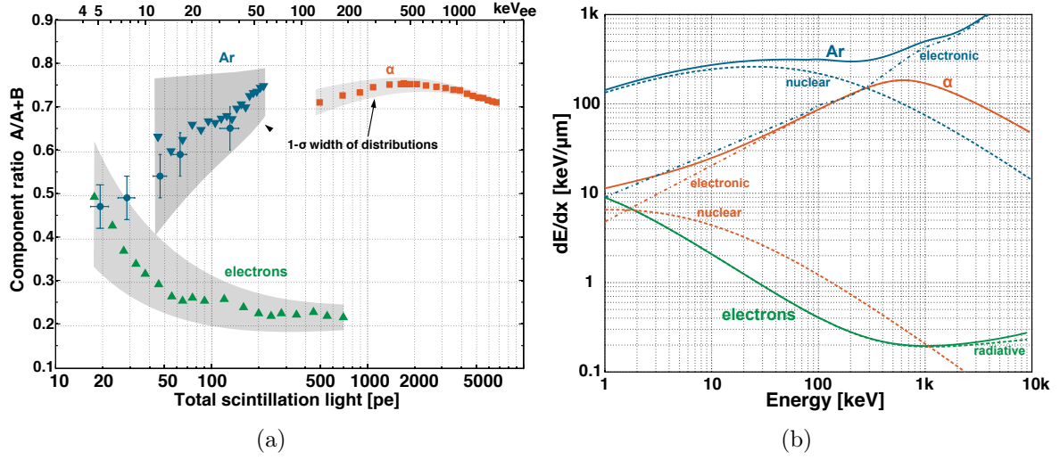
Figure 4.12: Left: CR vs. light yield for Ar, \alpha and e^- recoils. The grey zones indicate the 1- \sigma spread. Right: total stopping power (solid) and contributions (dashed) from SRIM, ASTAR and ESTAR [121].
